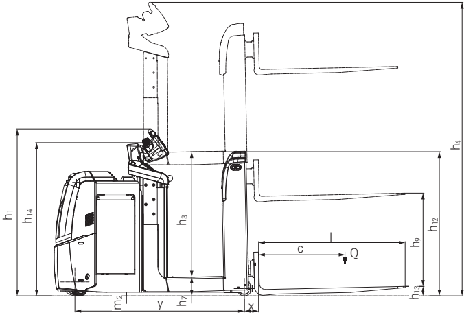
Side view OXV 08
