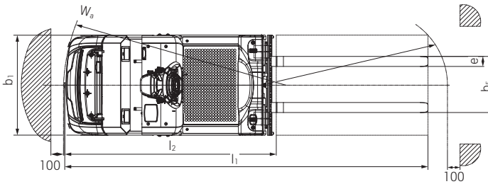
Top view OXV 08
